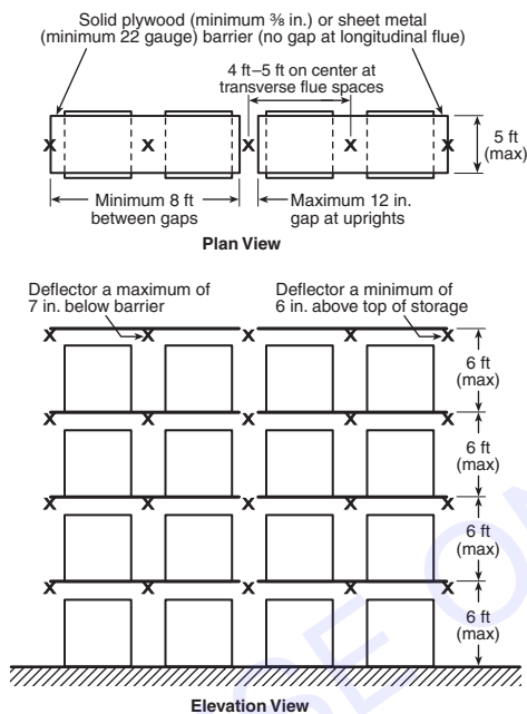
FIGURE 66.16.2.1(a) Single-Row Rack Sprinkler Layout for Design Scheme "B" — Sprinklers in Center of Rack. [30: Figure 16.6.2.1(a)]
