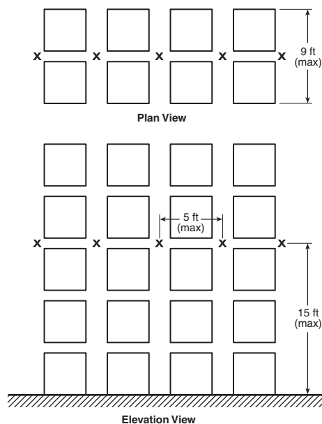
FIGURE 66.16.5(e) Double-Row Rack Sprinkler Layout H — Option #2. [30: Figure 16.6.5(e)]
