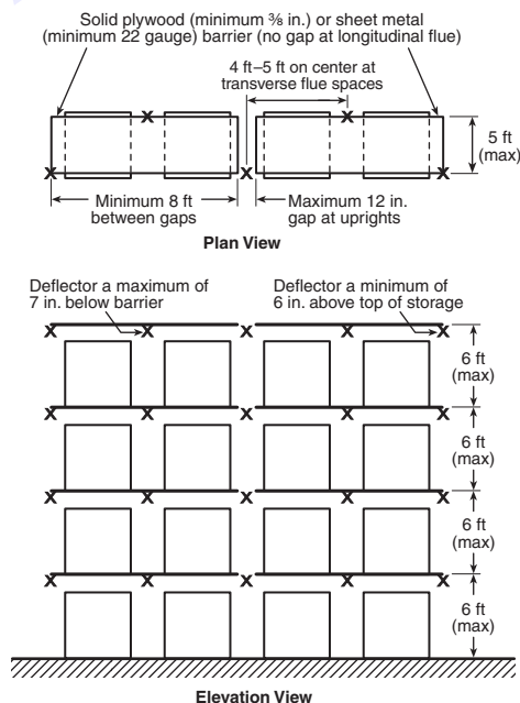
FIGURE 66.16.2.1(b) Single-Row Rack Sprinkler Layout for Design Scheme "B" — Sprinklers on Face of Rack. [30: Figure 16.6.2.1(b)]
